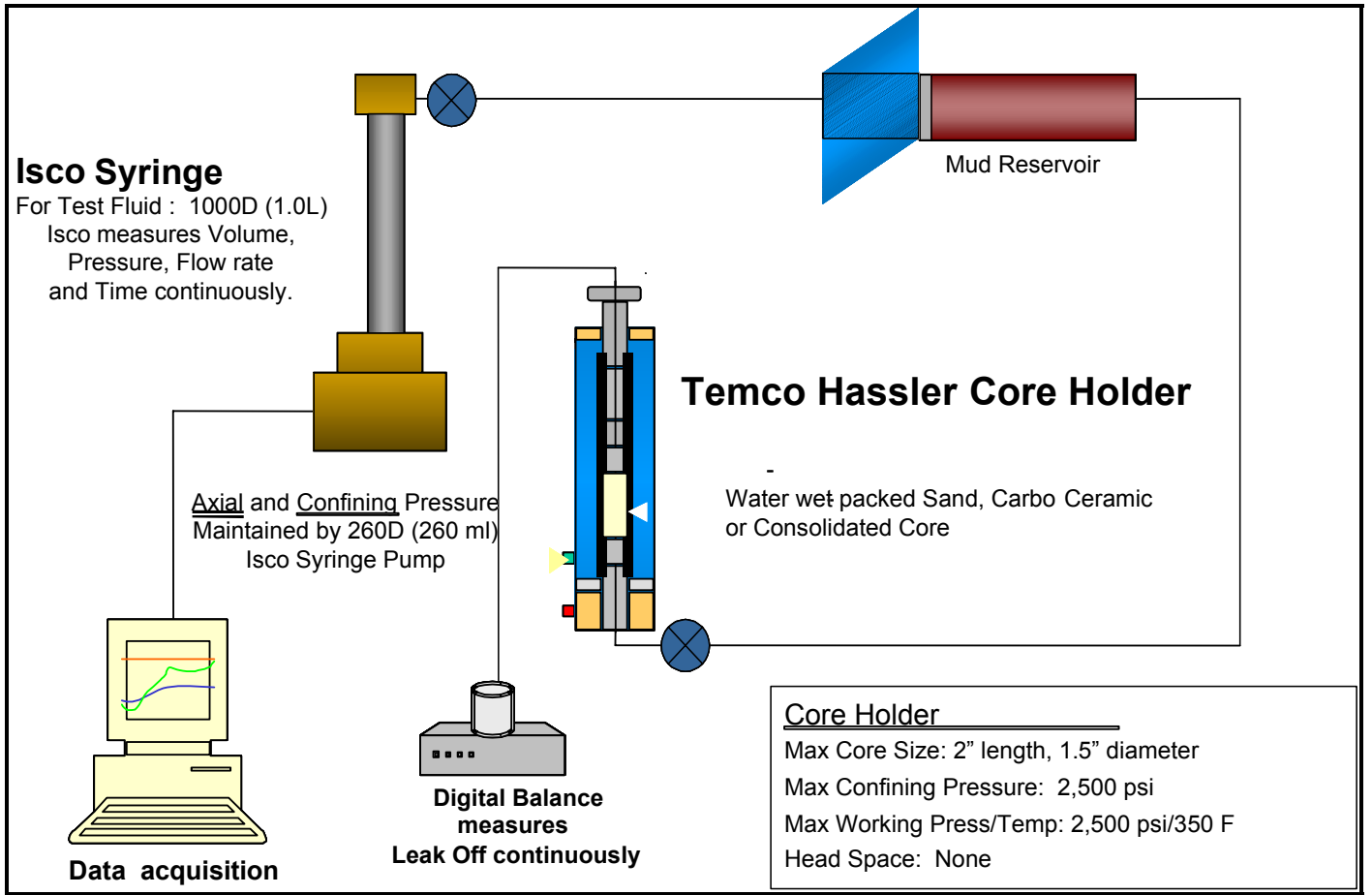
Fig. 2 Triaxial Coreholder for Sealing Tests.
