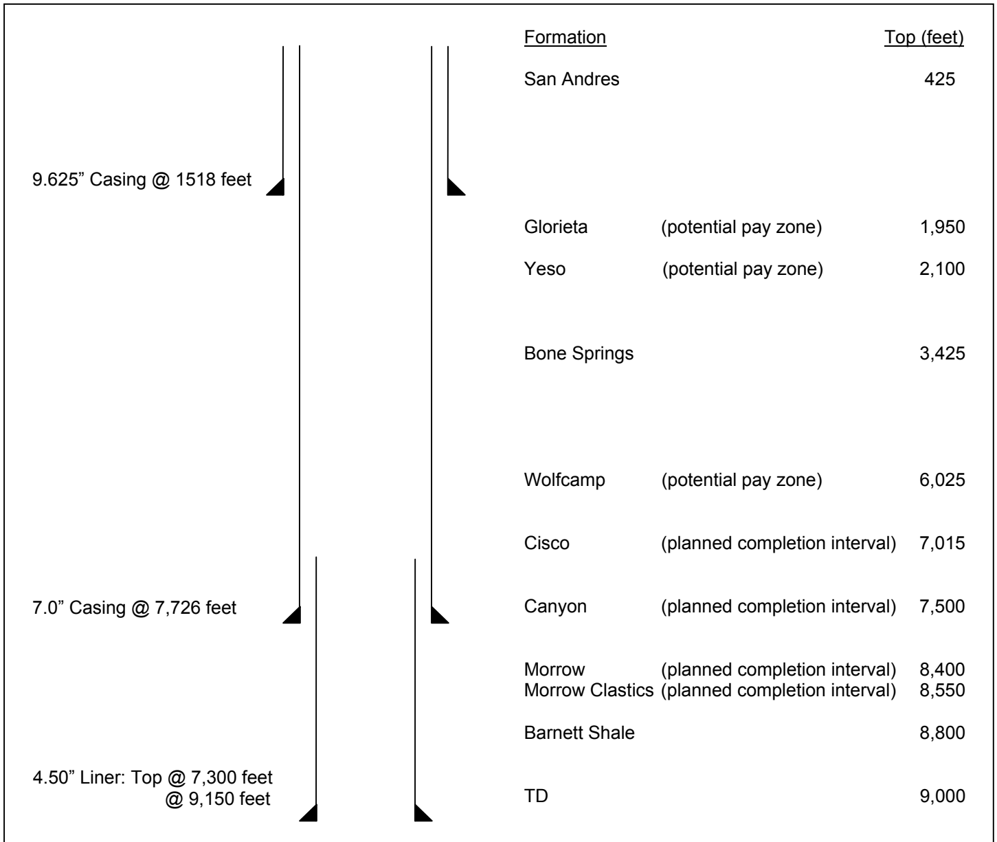
Fig. 5 Well Design and Estimated Formation Tops.
