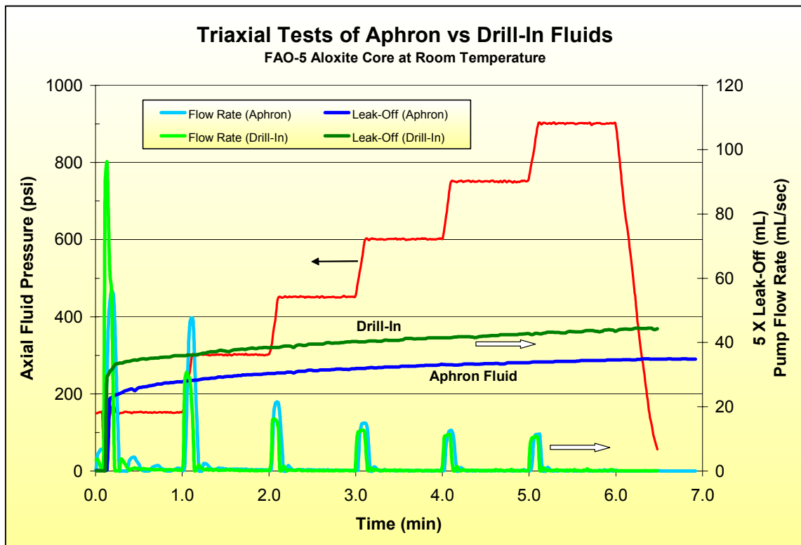
Aphrons-based versus typical Drill-In fluid sealing performance.
