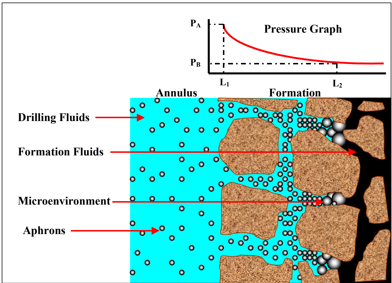
Fig. 1 Internal Seal and Pressure Graph.
