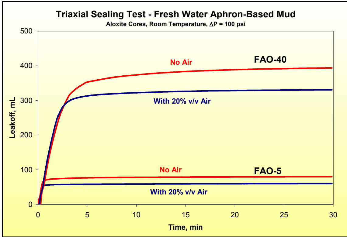
5-Darcy and 80-Darcy Aloxite core sealing with aphrons.
