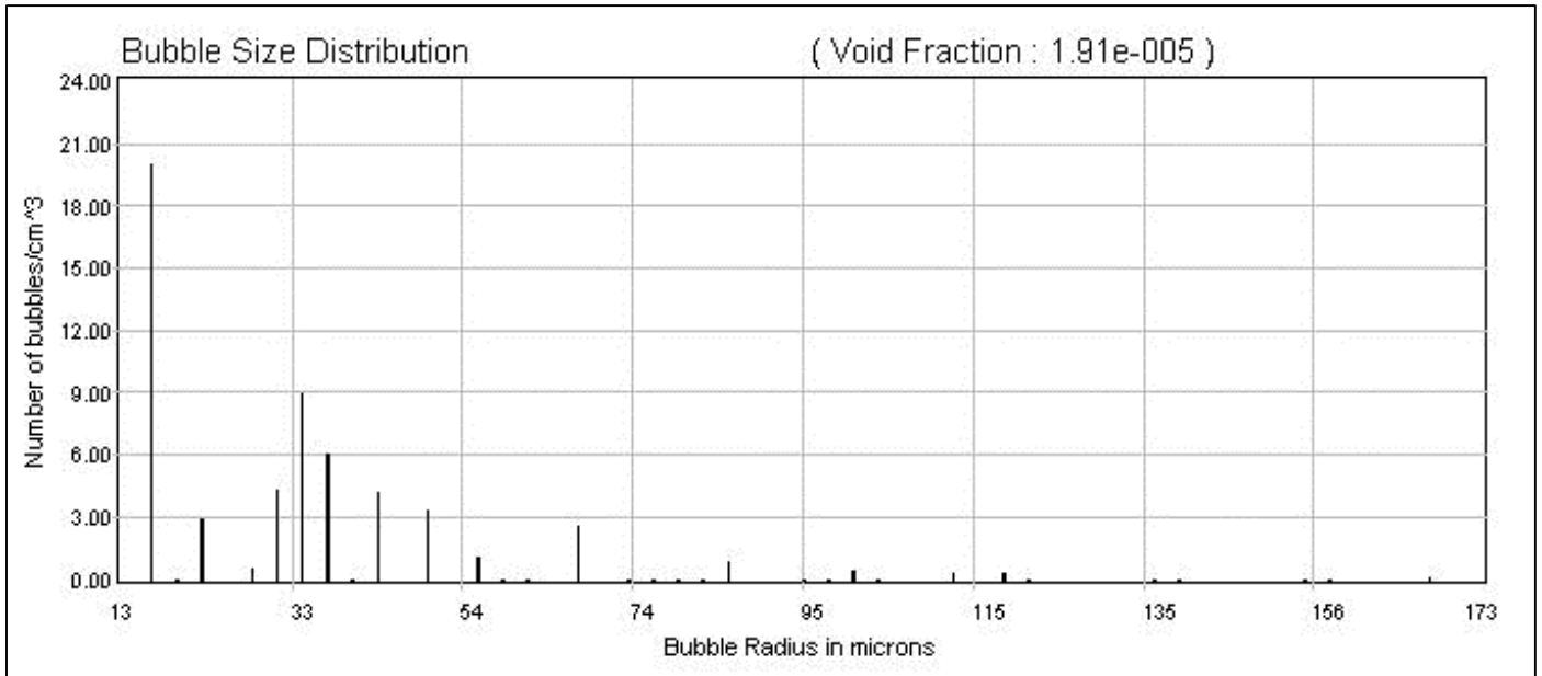
Fig. 3 Acoustic Bubble Spectrometer
